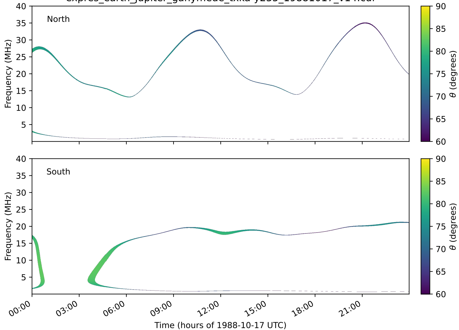
expres_earth_jupiter_ganymede_txka-y235_19881017_v14.cdf
