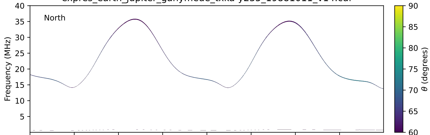
expres_earth_jupiter_ganymede_txka-y235_19881011_v14.cdf
