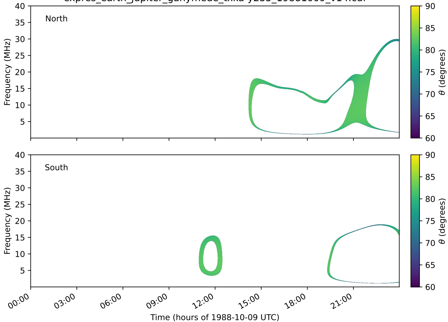
expres_earth_jupiter_ganymede_txka-y235_19881009_v14.cdf
