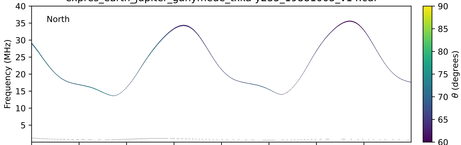
expres_earth_jupiter_ganymede_txka-y235_19881003_v14.cdf
