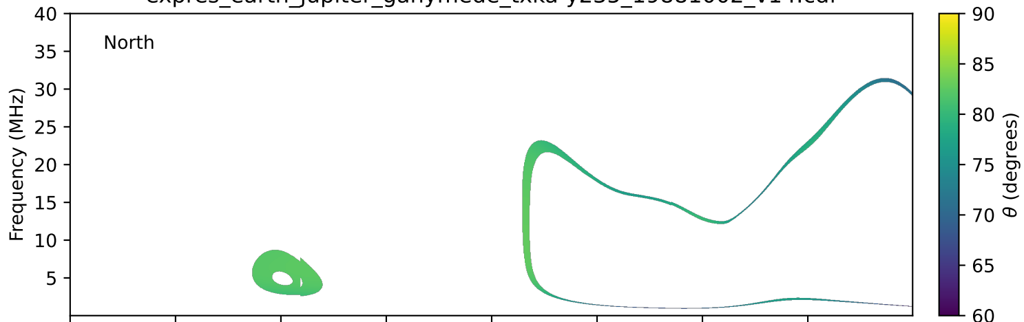
expres_earth_jupiter_ganymede_txka-y235_19881002_v14.cdf
