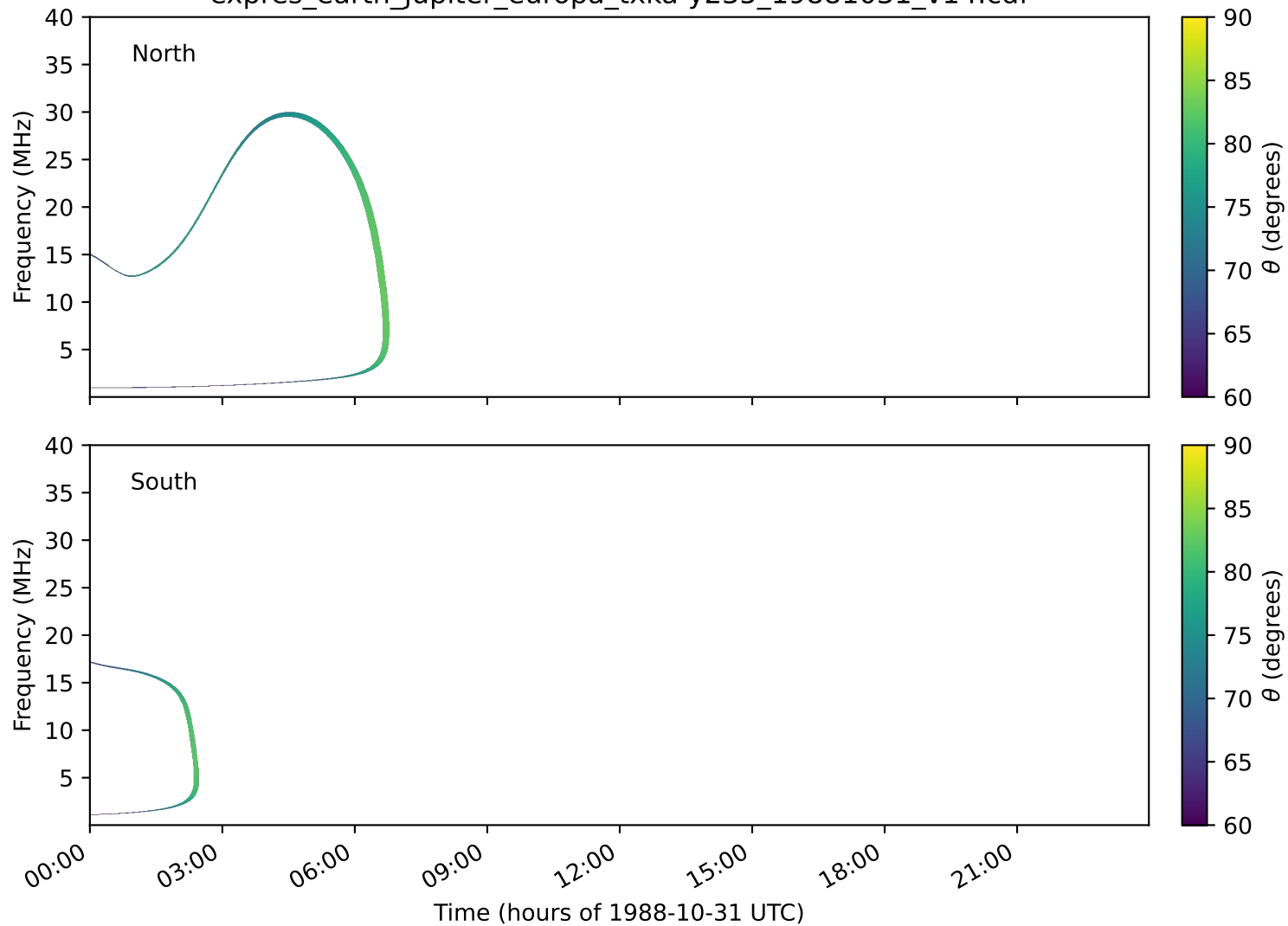
expres_earth_jupiter_europa_txka-y235_19881031_v14.cdf
