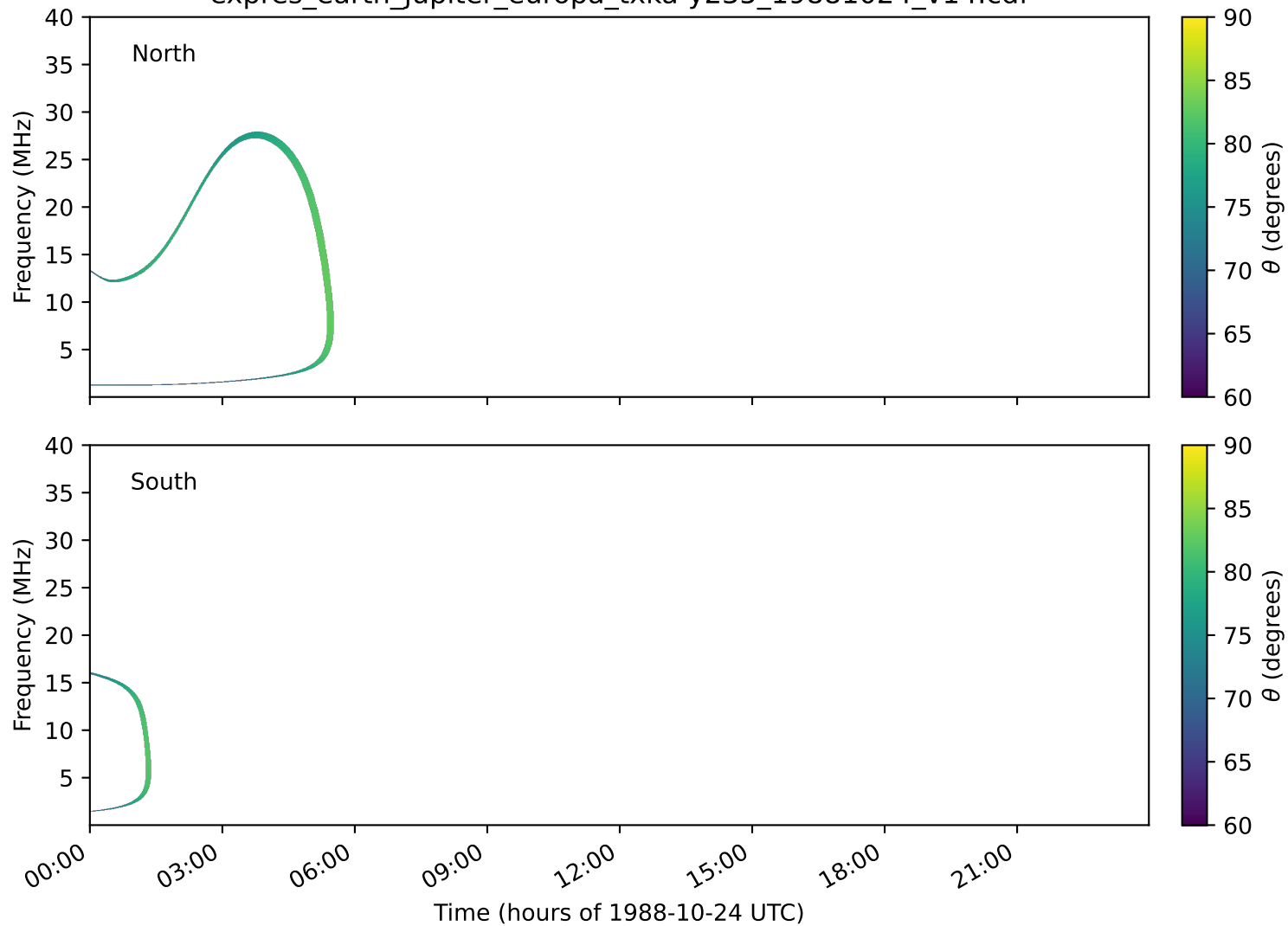
expres_earth_jupiter_europa_txka-y235_19881024_v14.cdf
