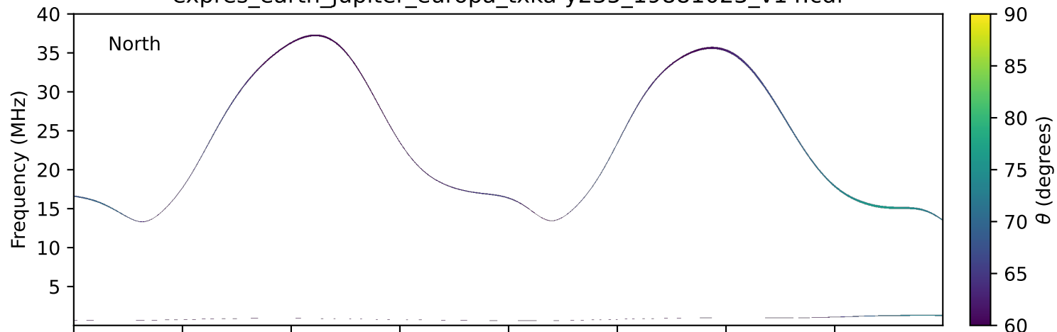
expres_earth_jupiter_europa_txka-y235_19881023_v14.cdf
