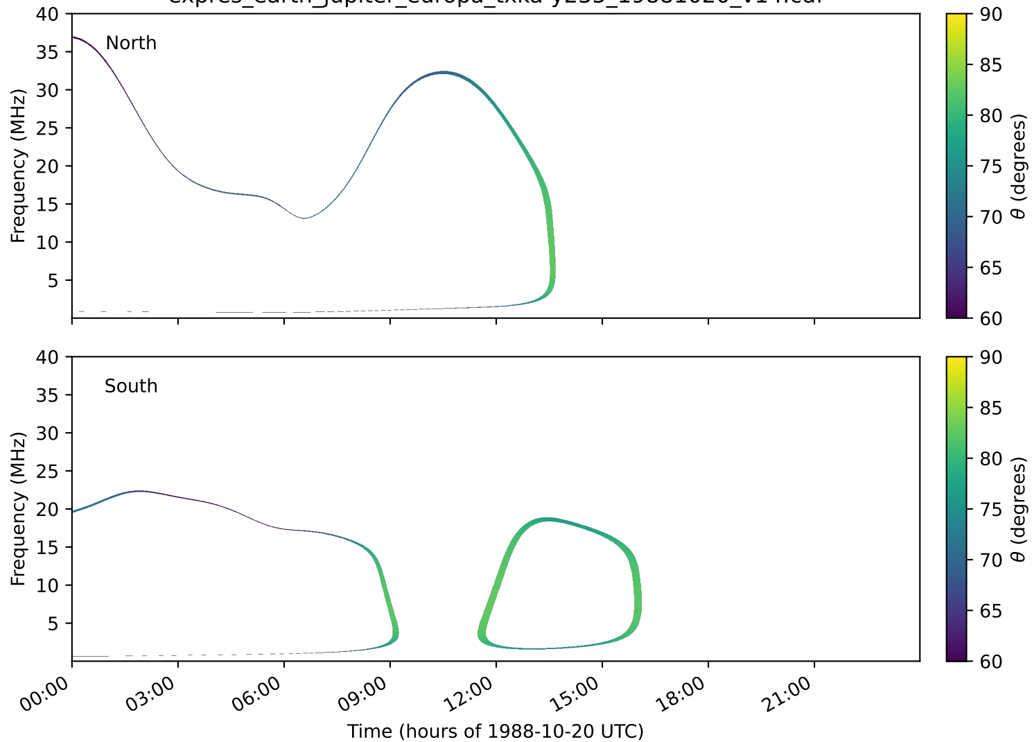
expres_earth_jupiter_europa_txka-y235_19881020_v14.cdf
