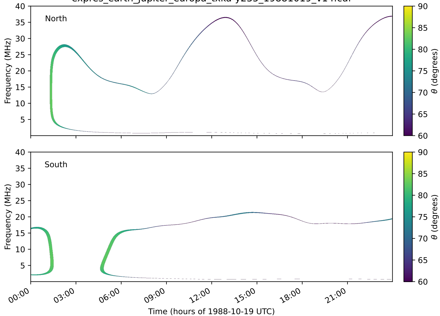
expres_earth_jupiter_europa_txka-y235_19881019_v14.cdf
