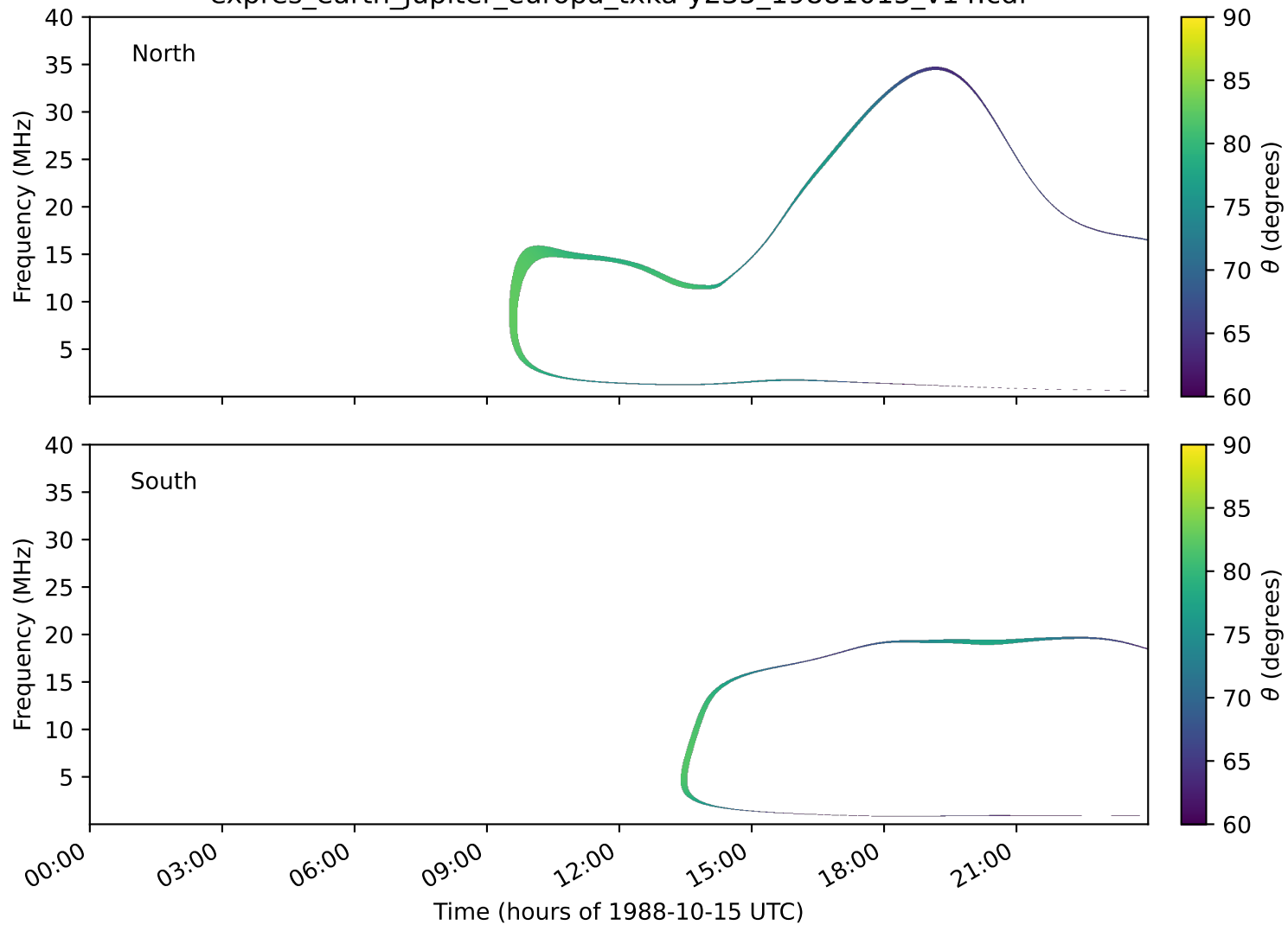
expres_earth_jupiter_europa_txka-y235_19881015_v14.cdf
