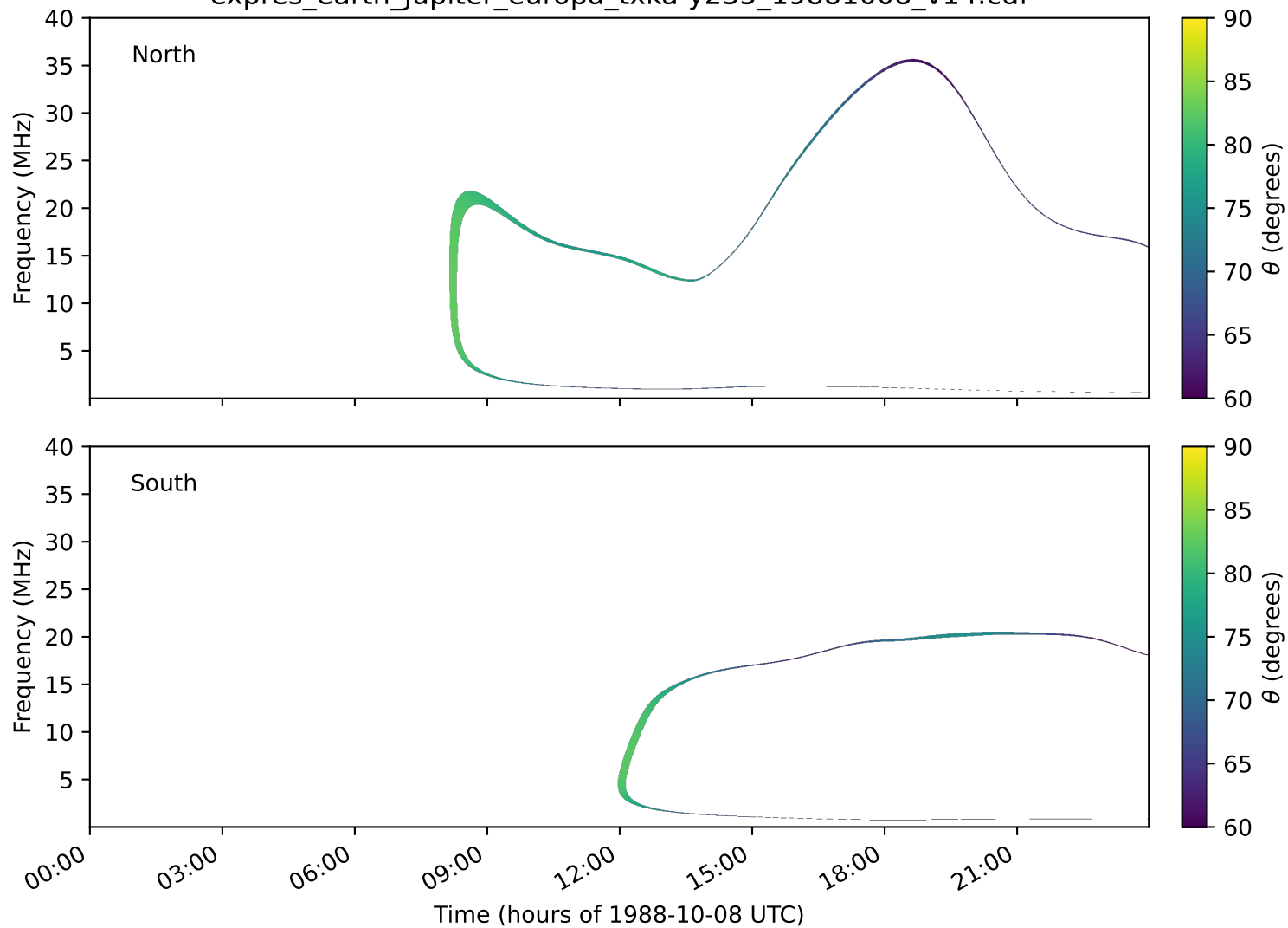
expres_earth_jupiter_europa_txka-y235_19881008_v14.cdf
