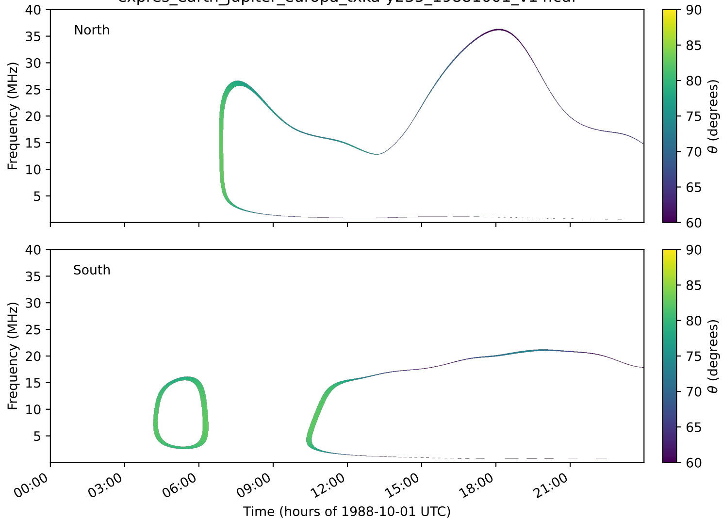
expres_earth_jupiter_europa_txka-y235_19881001_v14.cdf
