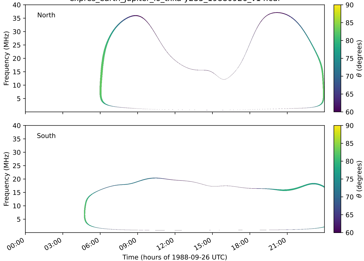
expres_earth_jupiter_io_txka-y235_19880926_v14.cdf
