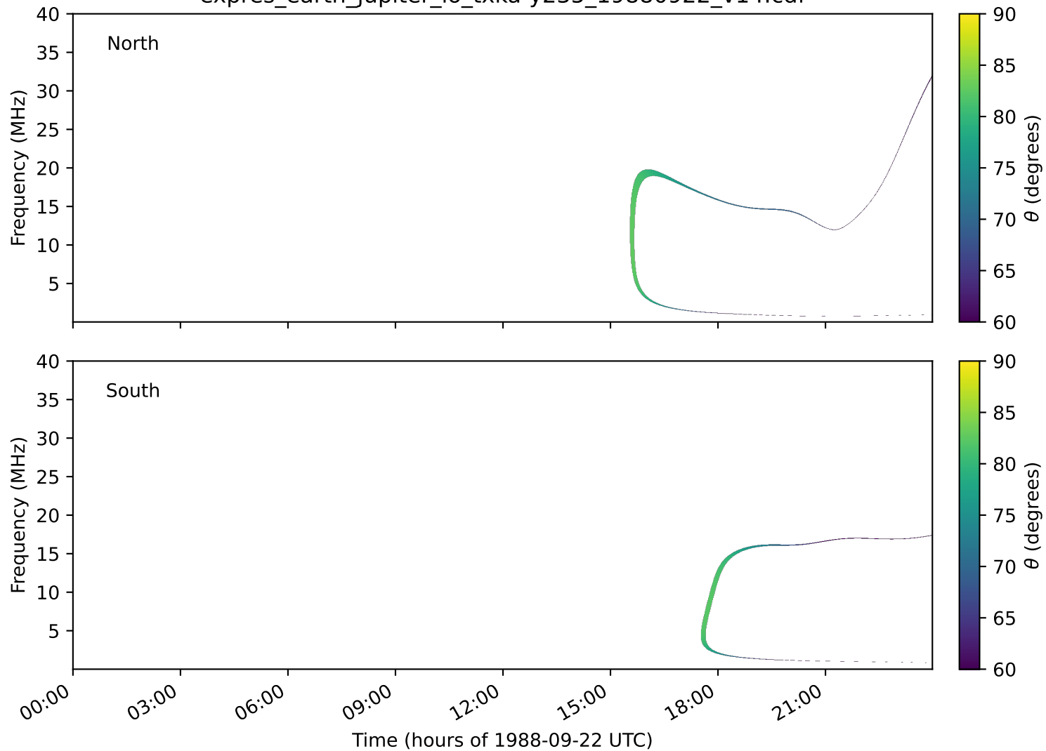
expres_earth_jupiter_io_txka-y235_19880922_v14.cdf
