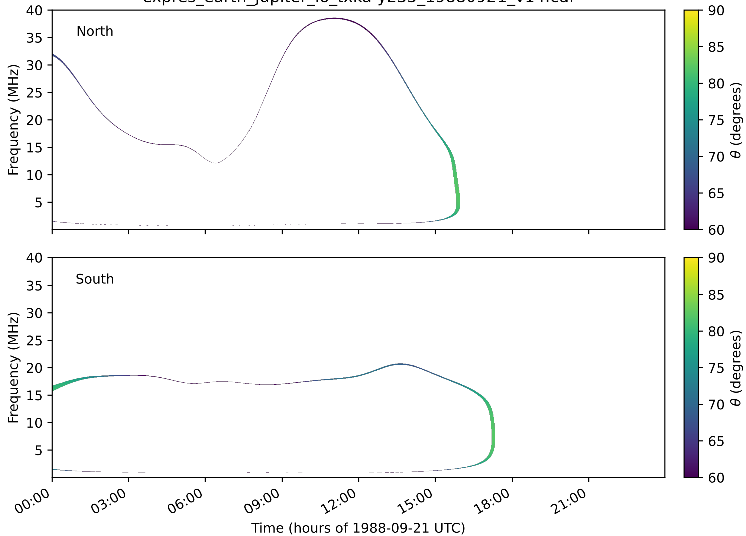
expres_earth_jupiter_io_txka-y235_19880921_v14.cdf
