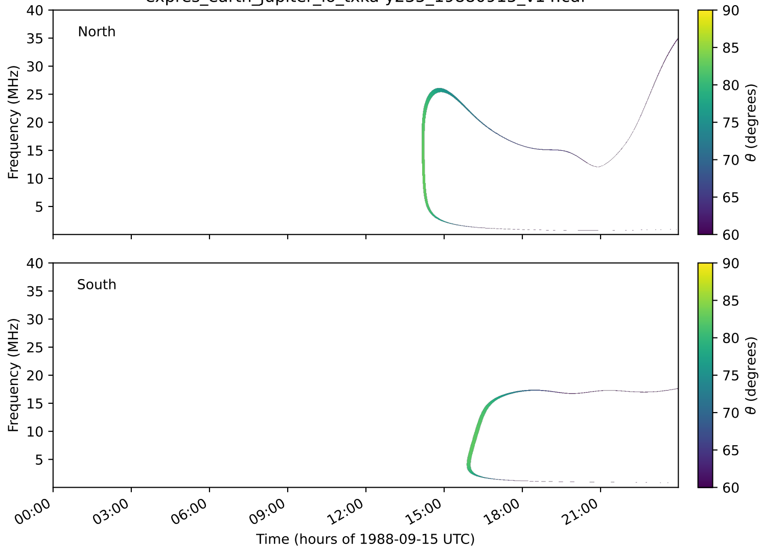
expres_earth_jupiter_io_txka-y235_19880915_v14.cdf
