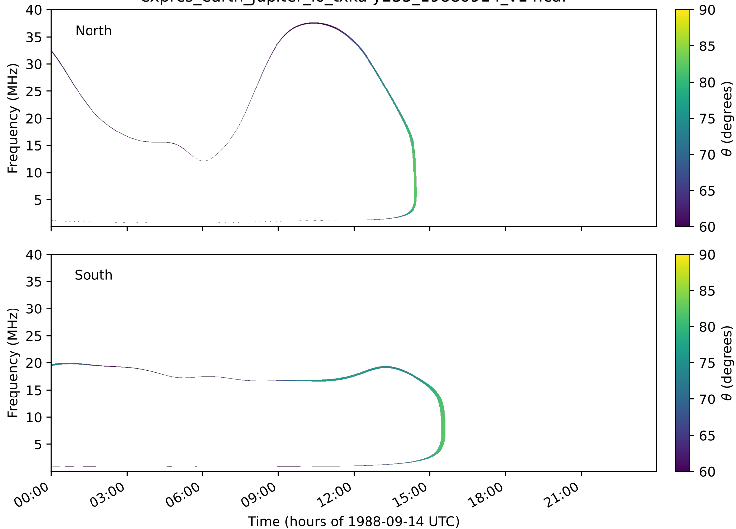
expres_earth_jupiter_io_txka-y235_19880914_v14.cdf
