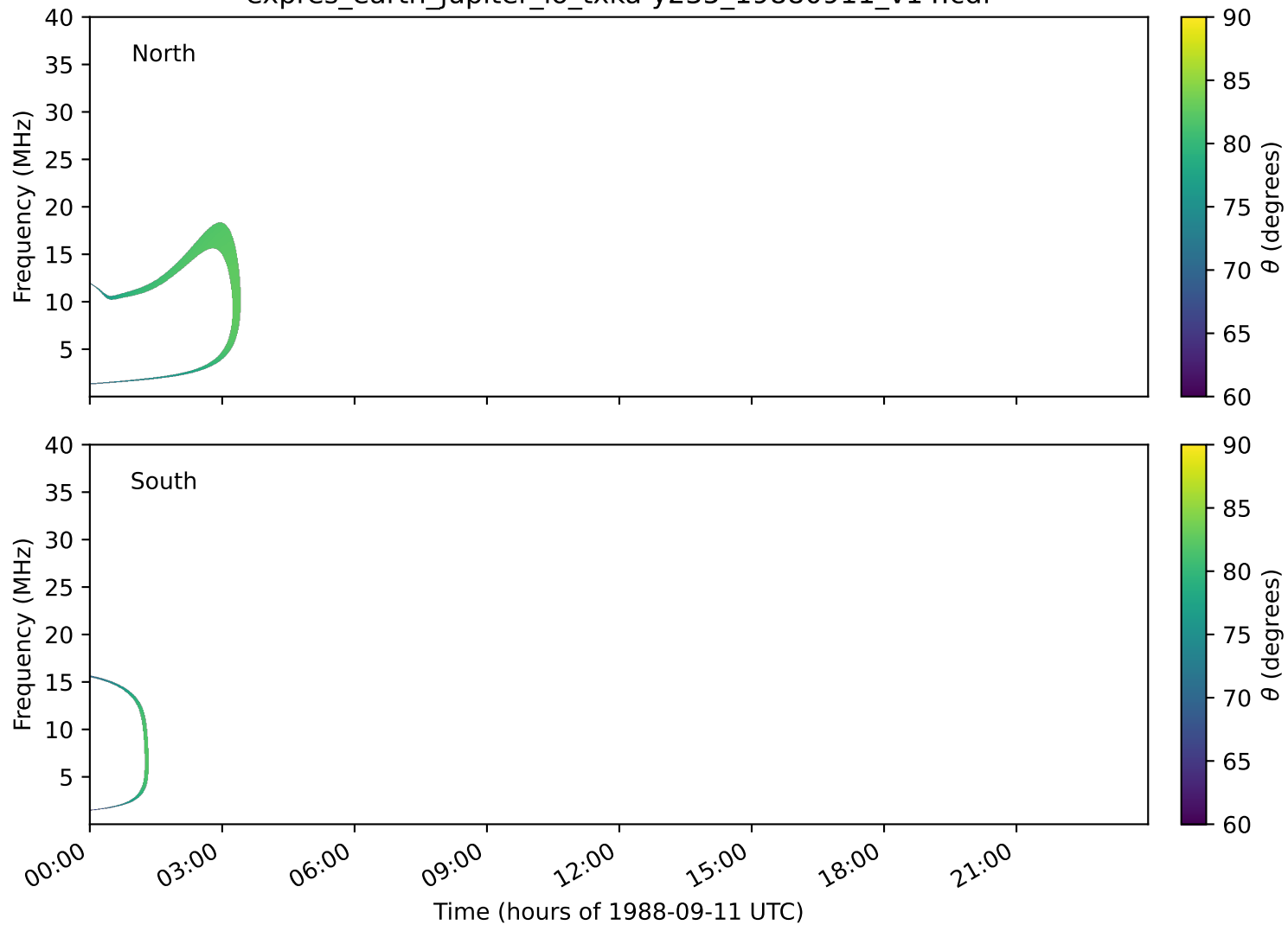
expres_earth_jupiter_io_txka-y235_19880911_v14.cdf
