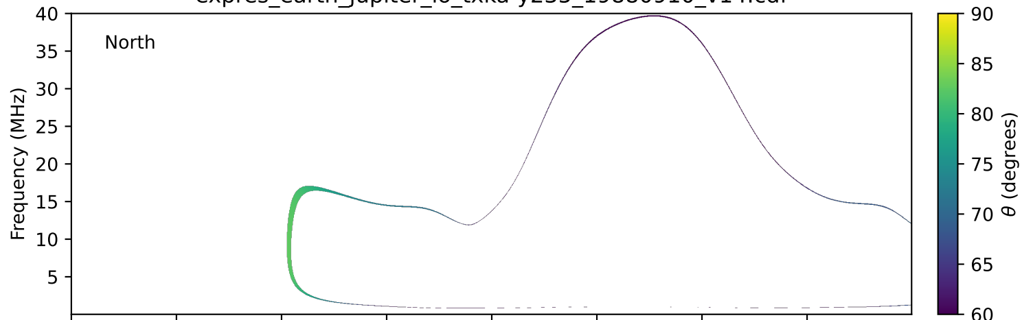
expres_earth_jupiter_io_txka-y235_19880910_v14.cdf
