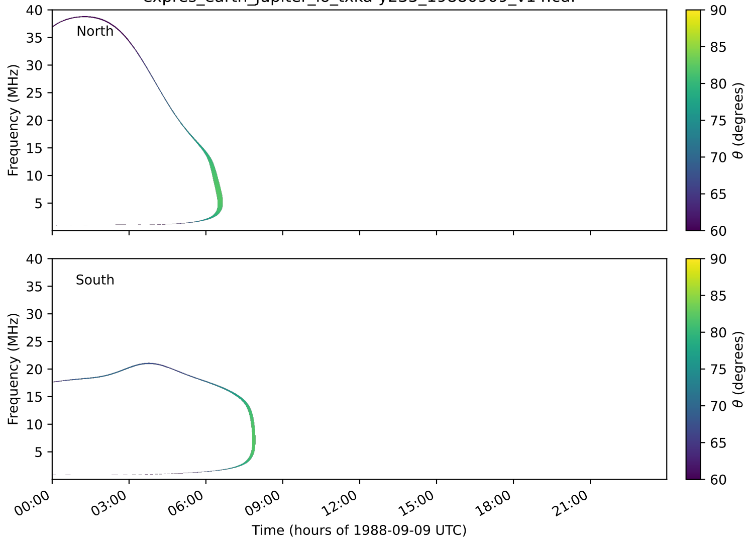
expres_earth_jupiter_io_txka-y235_19880909_v14.cdf
