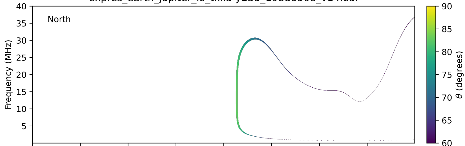
expres_earth_jupiter_io_txka-y235_19880908_v14.cdf
