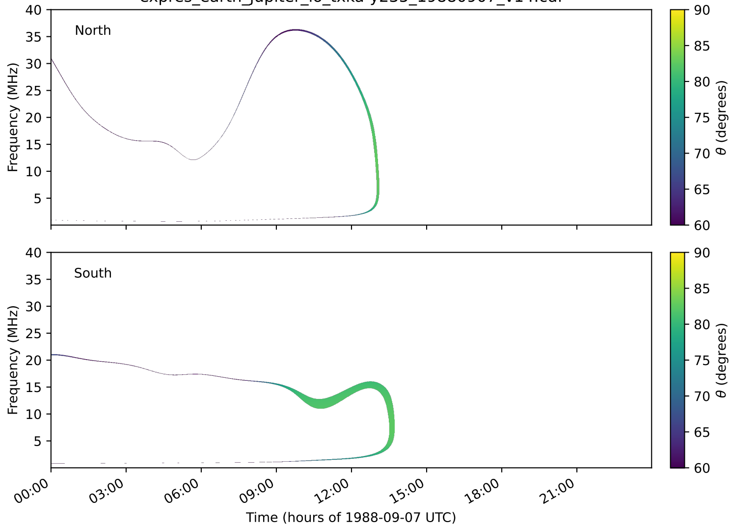
expres_earth_jupiter_io_txka-y235_19880907_v14.cdf
