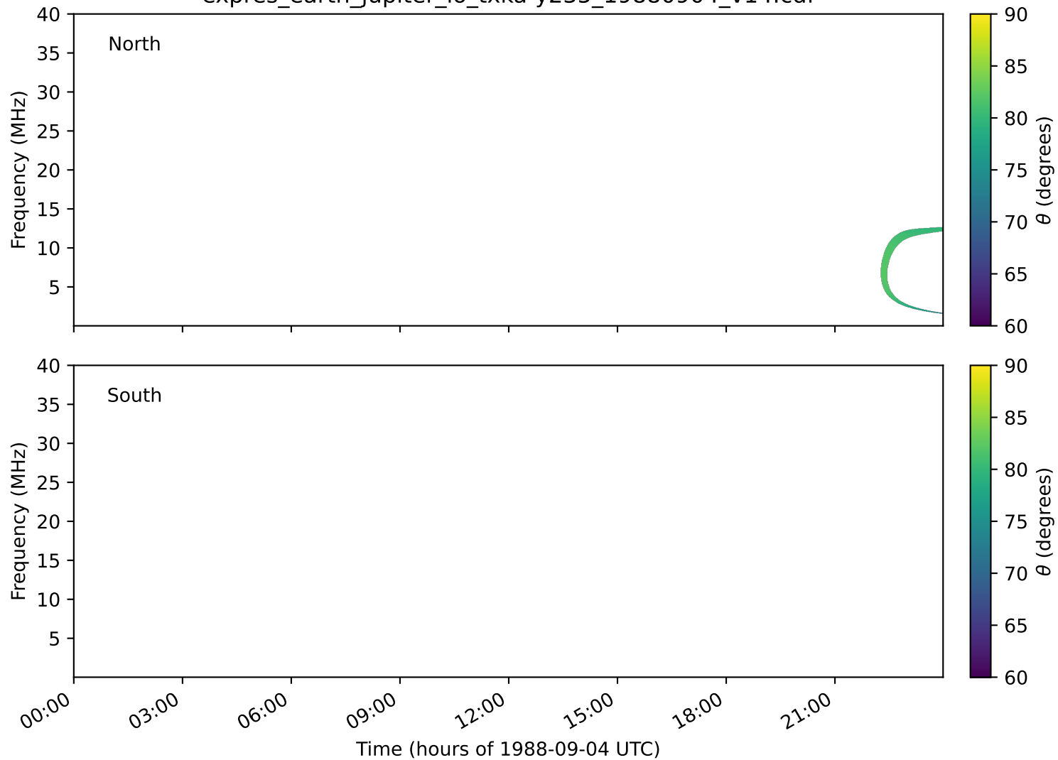
expres_earth_jupiter_io_txka-y235_19880904_v14.cdf
