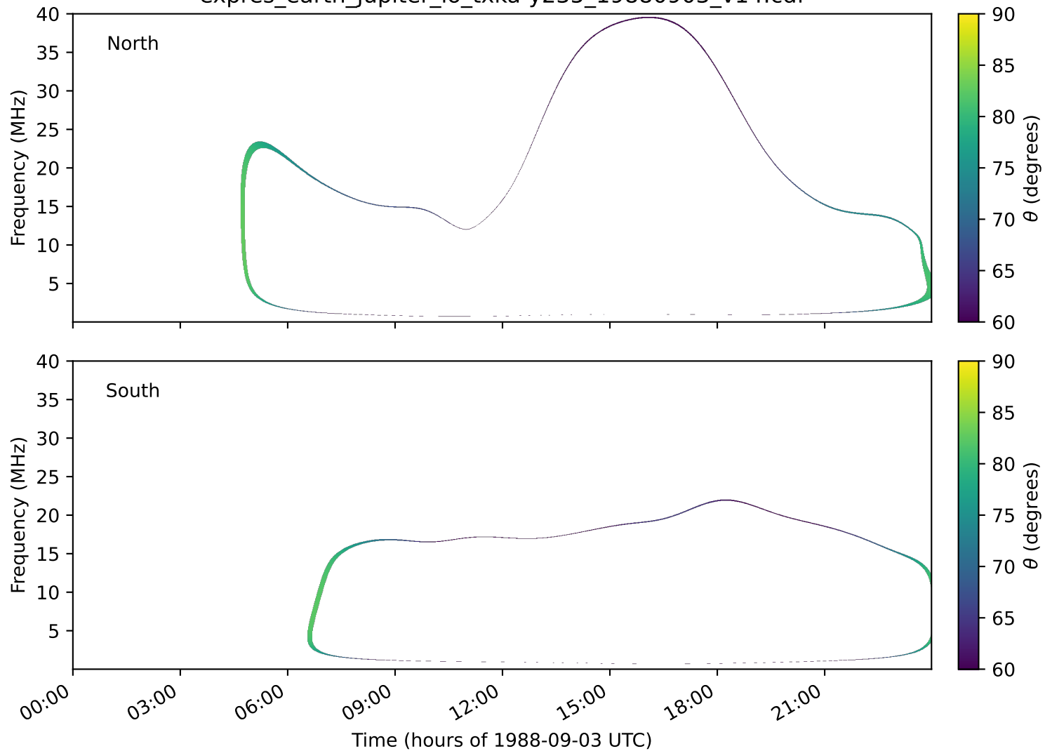
expres_earth_jupiter_io_txka-y235_19880903_v14.cdf
