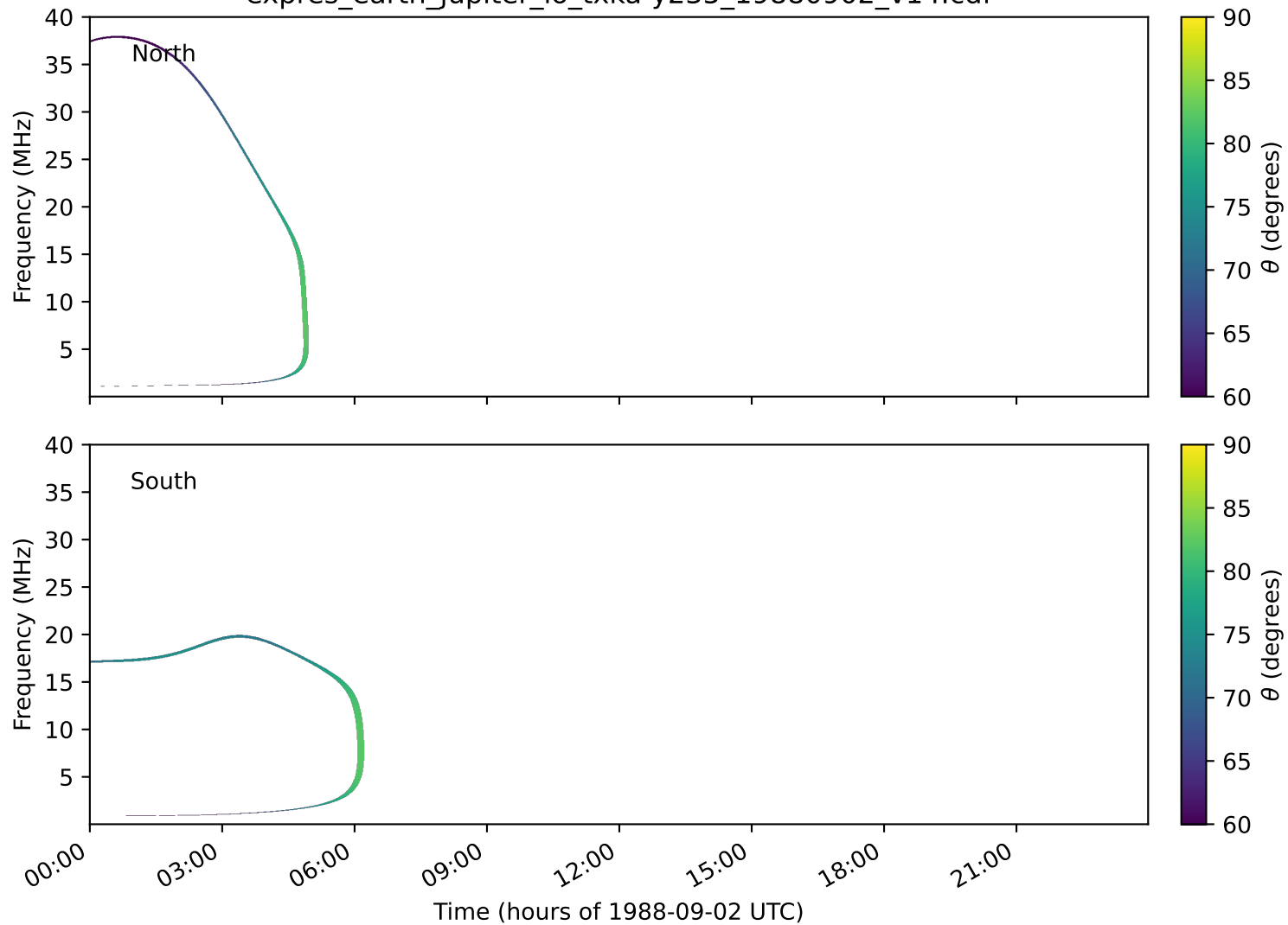
expres_earth_jupiter_io_txka-y235_19880902_v14.cdf
