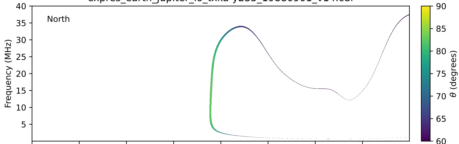
expres_earth_jupiter_io_txka-y235_19880901_v14.cdf
