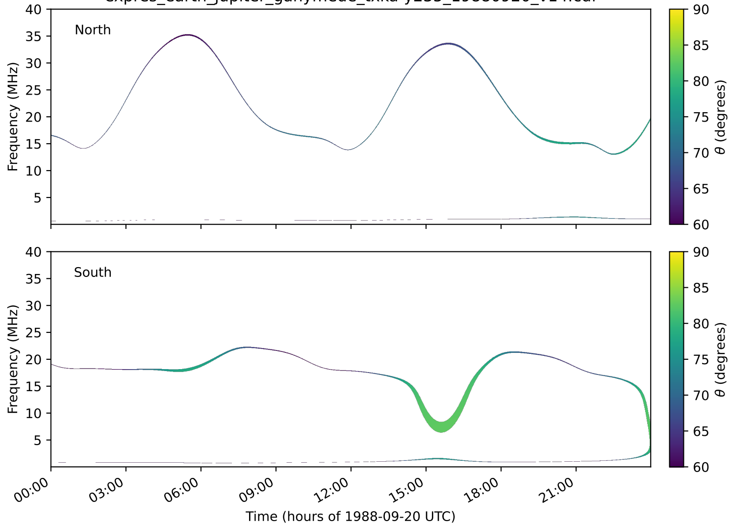
expres_earth_jupiter_ganymede_txka-y235_19880920_v14.cdf
