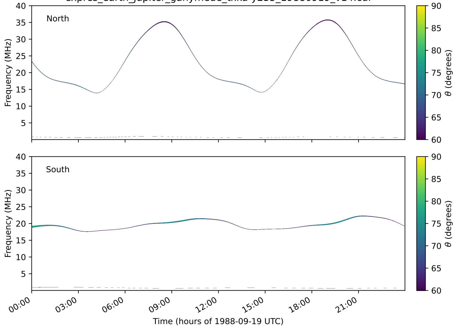
expres_earth_jupiter_ganymede_txka-y235_19880919_v14.cdf
