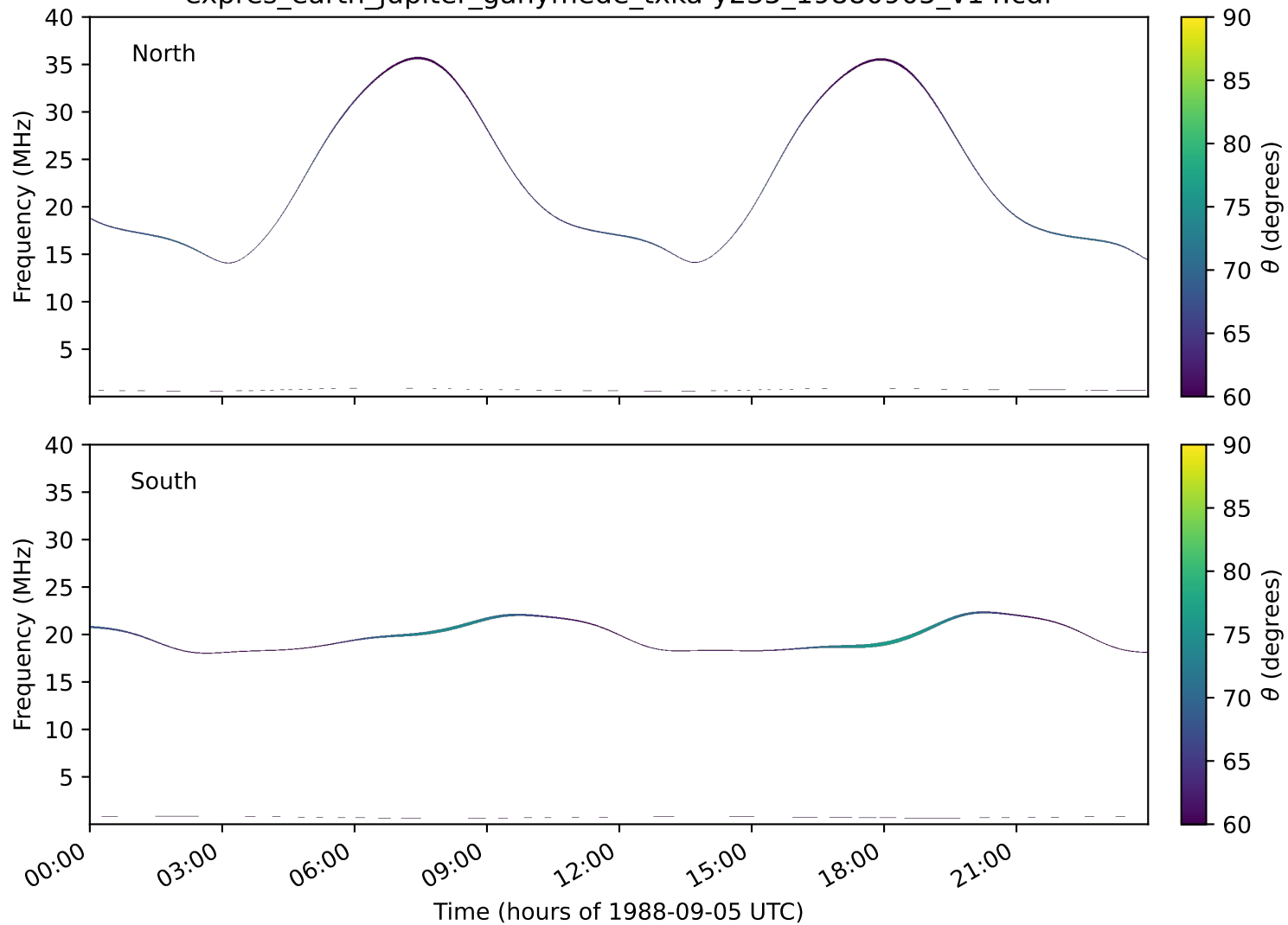
expres_earth_jupiter_ganymede_txka-y235_19880905_v14.cdf
