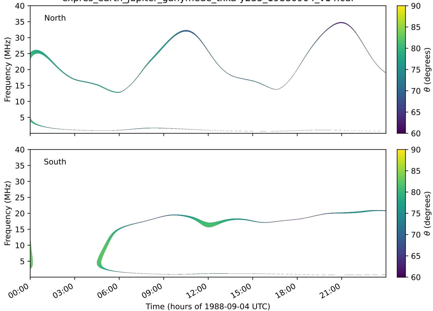
expres_earth_jupiter_ganymede_txka-y235_19880904_v14.cdf
