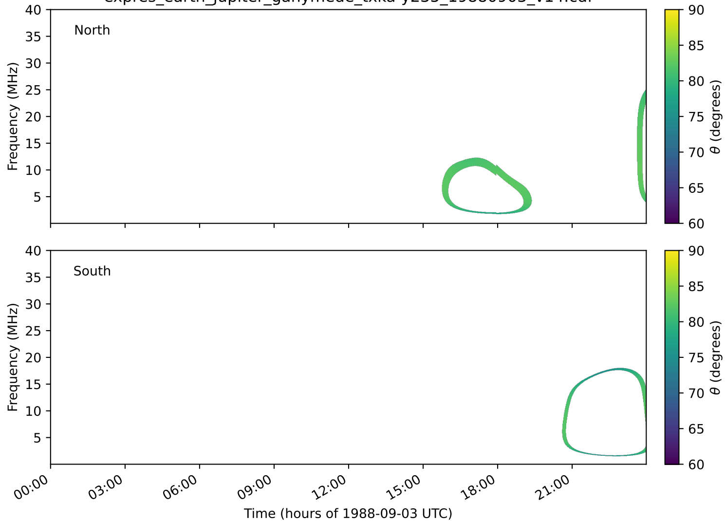
expres_earth_jupiter_ganymede_txka-y235_19880903_v14.cdf
