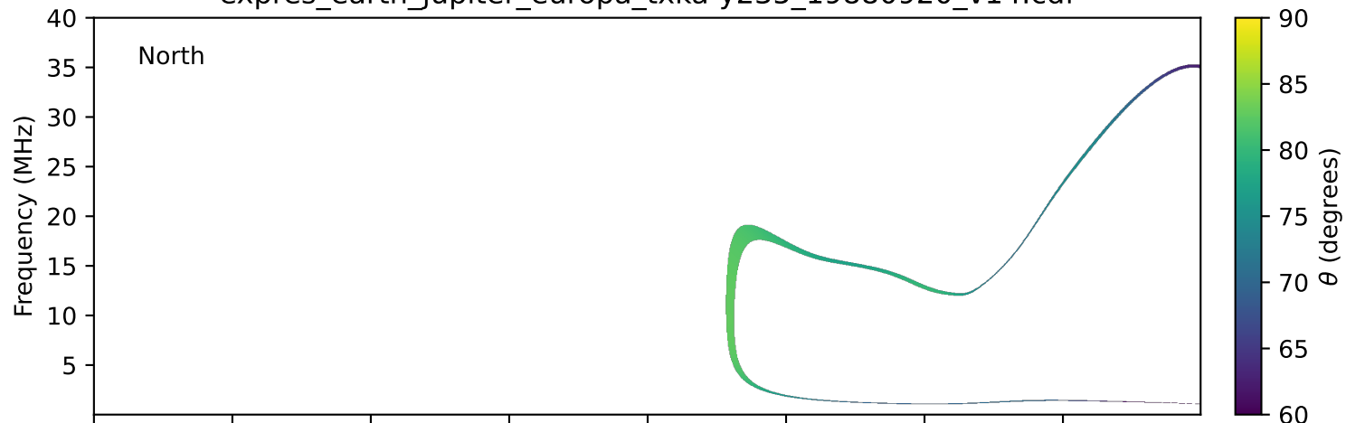
expres_earth_jupiter_europa_txka-y235_19880920_v14.cdf
