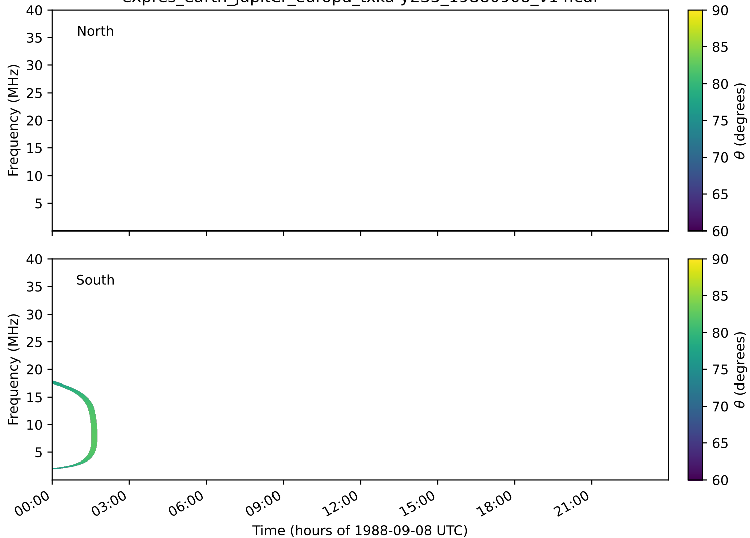
expres_earth_jupiter_europa_txka-y235_19880908_v14.cdf
