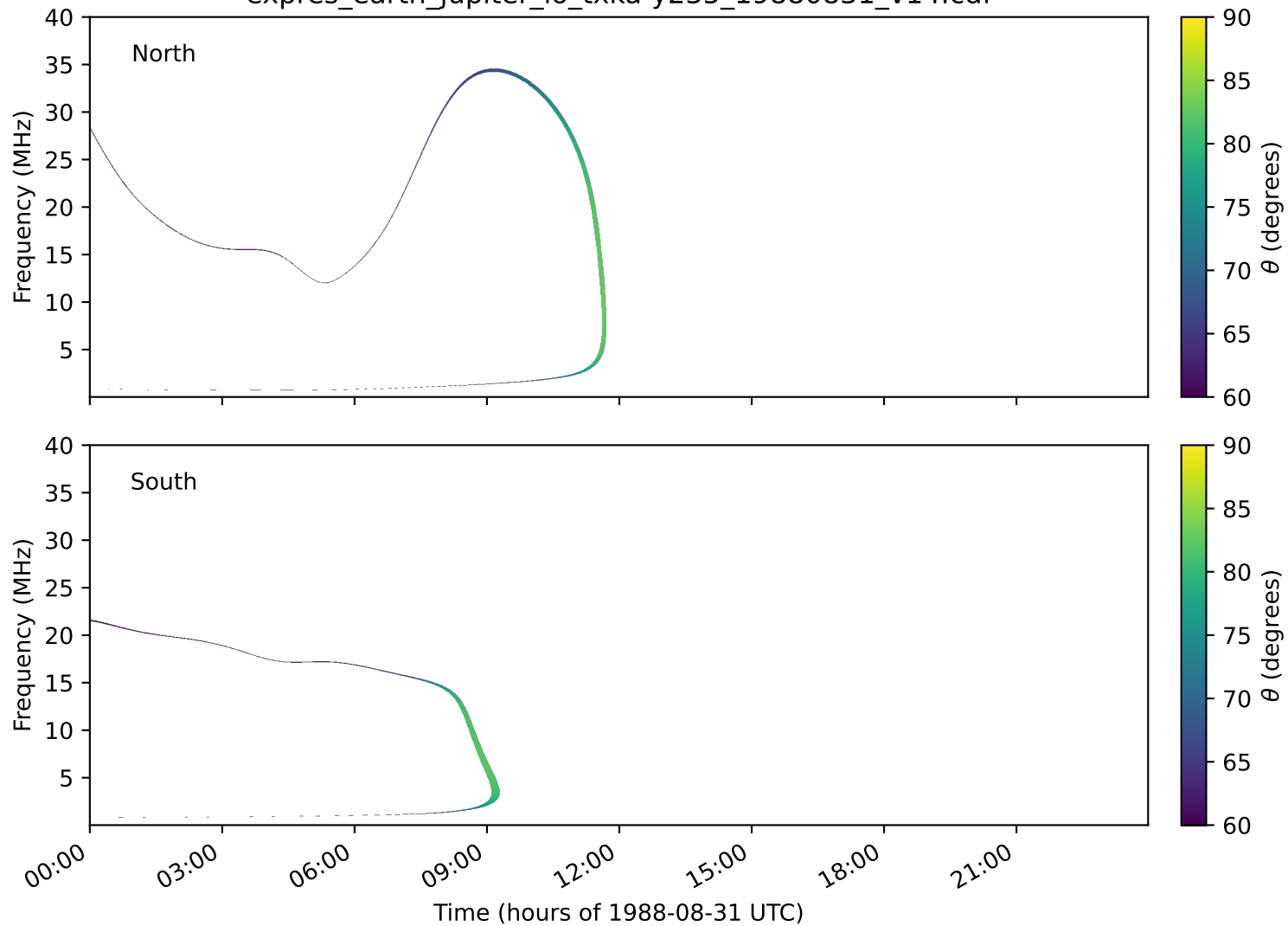
expres_earth_jupiter_io_txka-y235_19880831_v14.cdf
