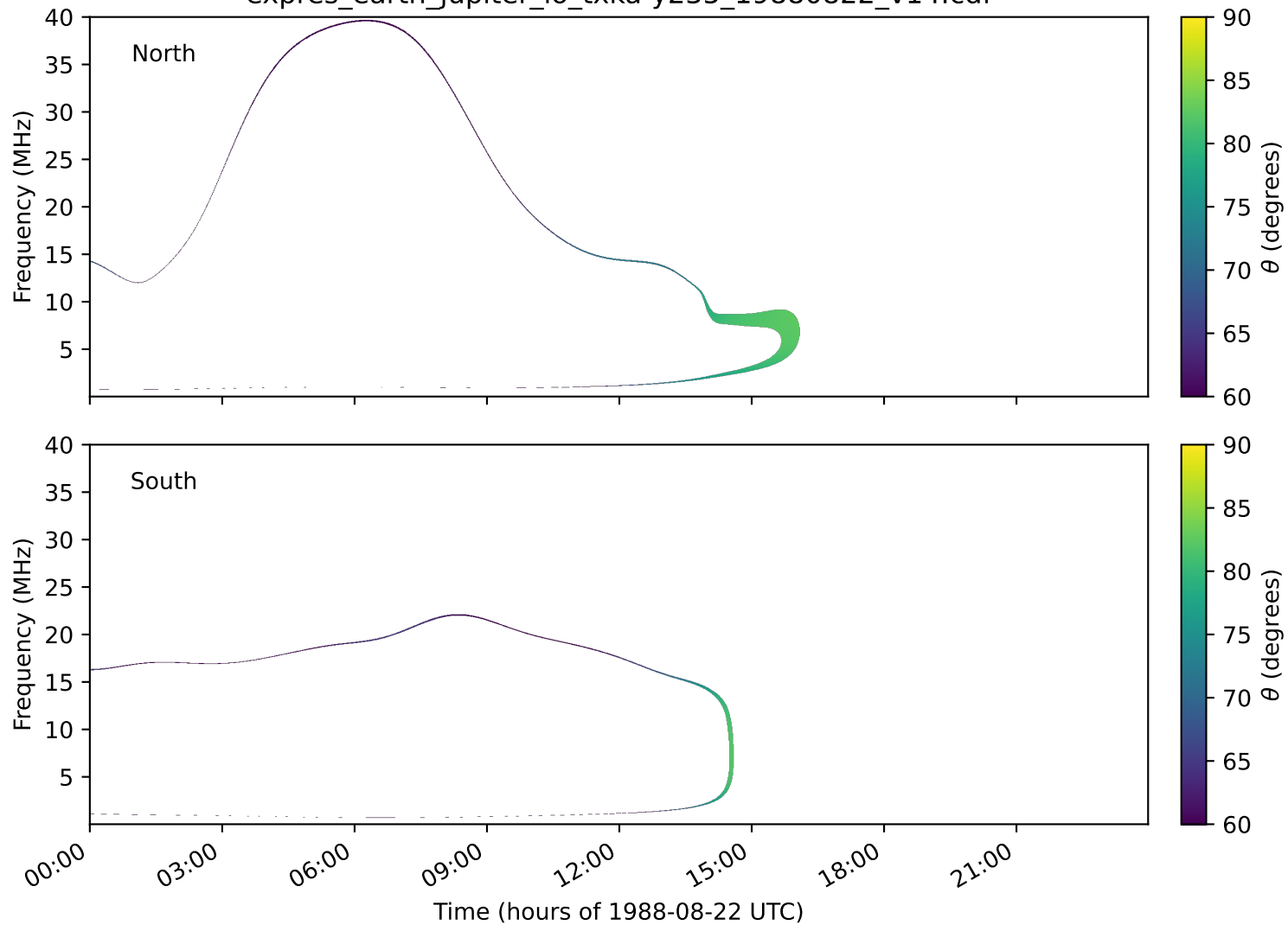
expres_earth_jupiter_io_txka-y235_19880822_v14.cdf
