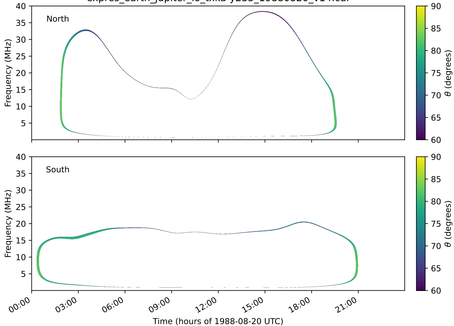
expres_earth_jupiter_io_txka-y235_19880820_v14.cdf
