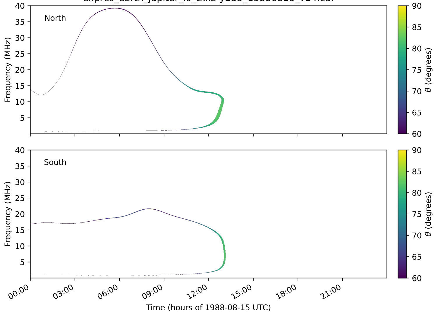
expres_earth_jupiter_io_txka-y235_19880815_v14.cdf
