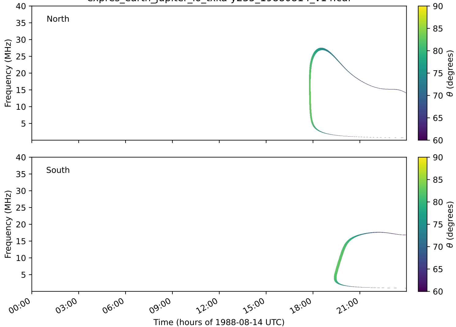
expres_earth_jupiter_io_txka-y235_19880814_v14.cdf
