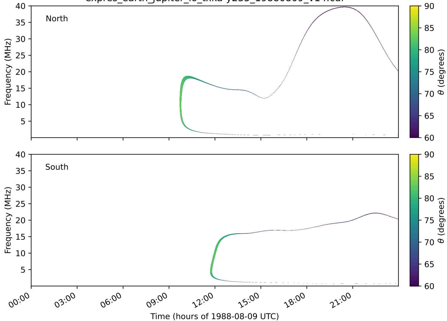
expres_earth_jupiter_io_txka-y235_19880809_v14.cdf
