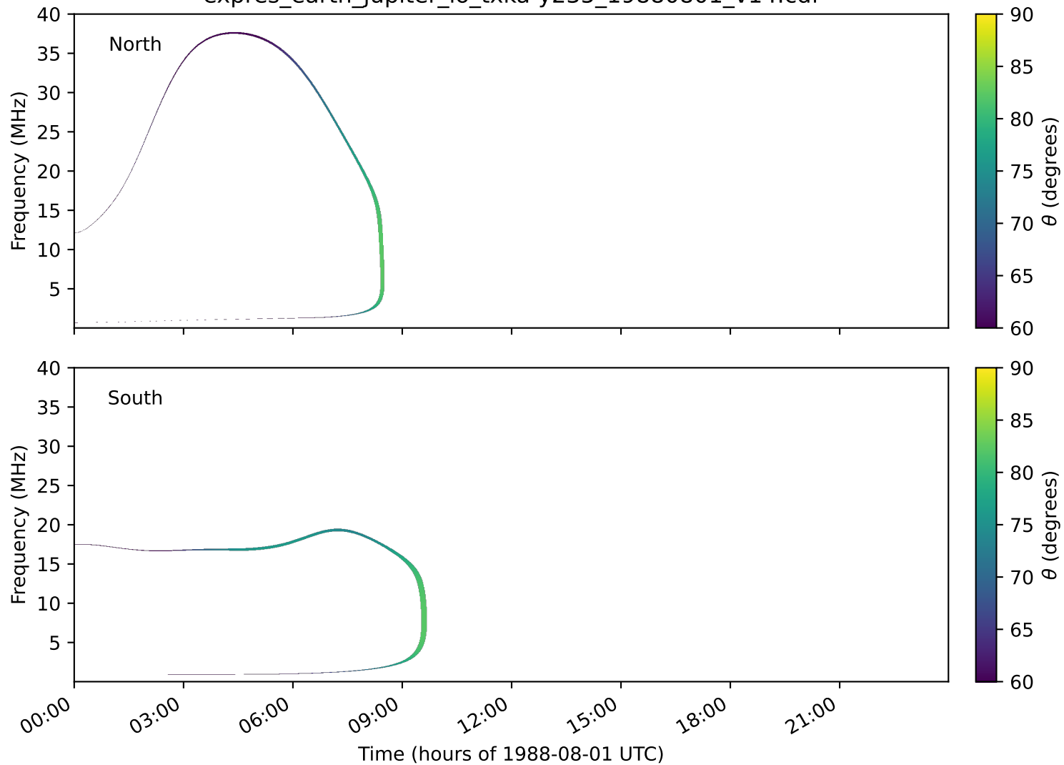
expres_earth_jupiter_io_txka-y235_19880801_v14.cdf
