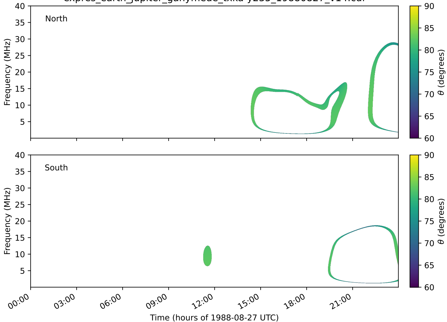
expres_earth_jupiter_ganymede_txka-y235_19880827_v14.cdf
