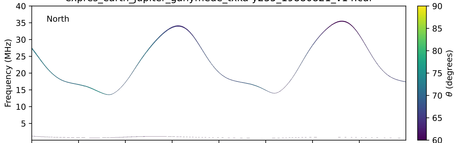
expres_earth_jupiter_ganymede_txka-y235_19880821_v14.cdf
