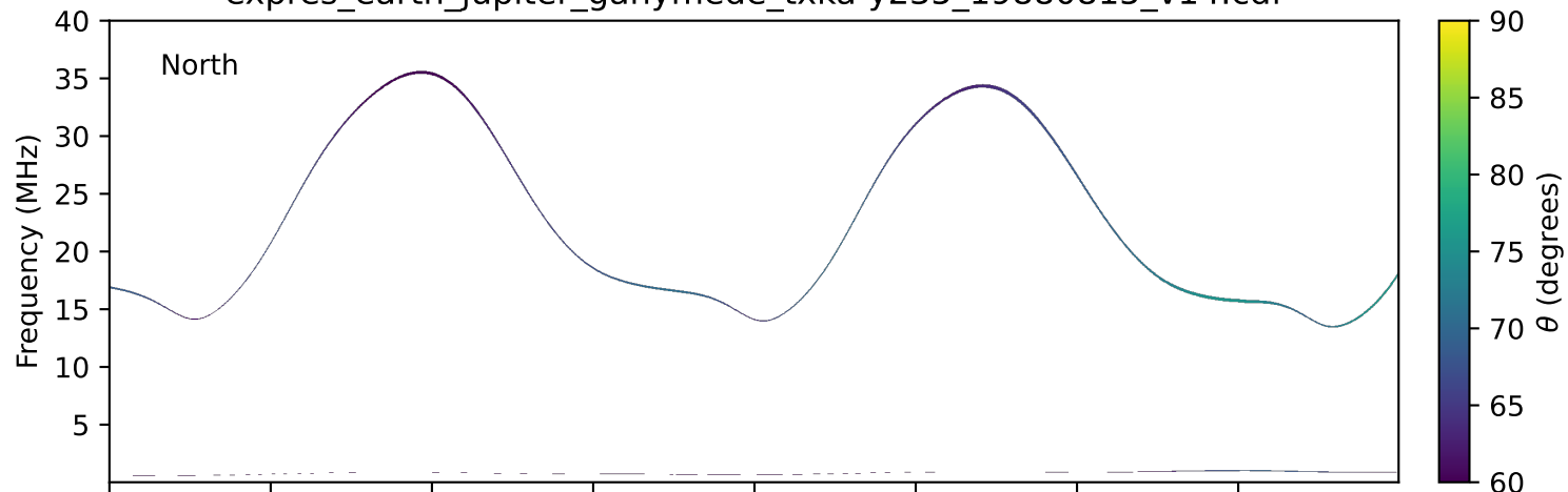
expres_earth_jupiter_ganymede_txka-y235_19880815_v14.cdf
