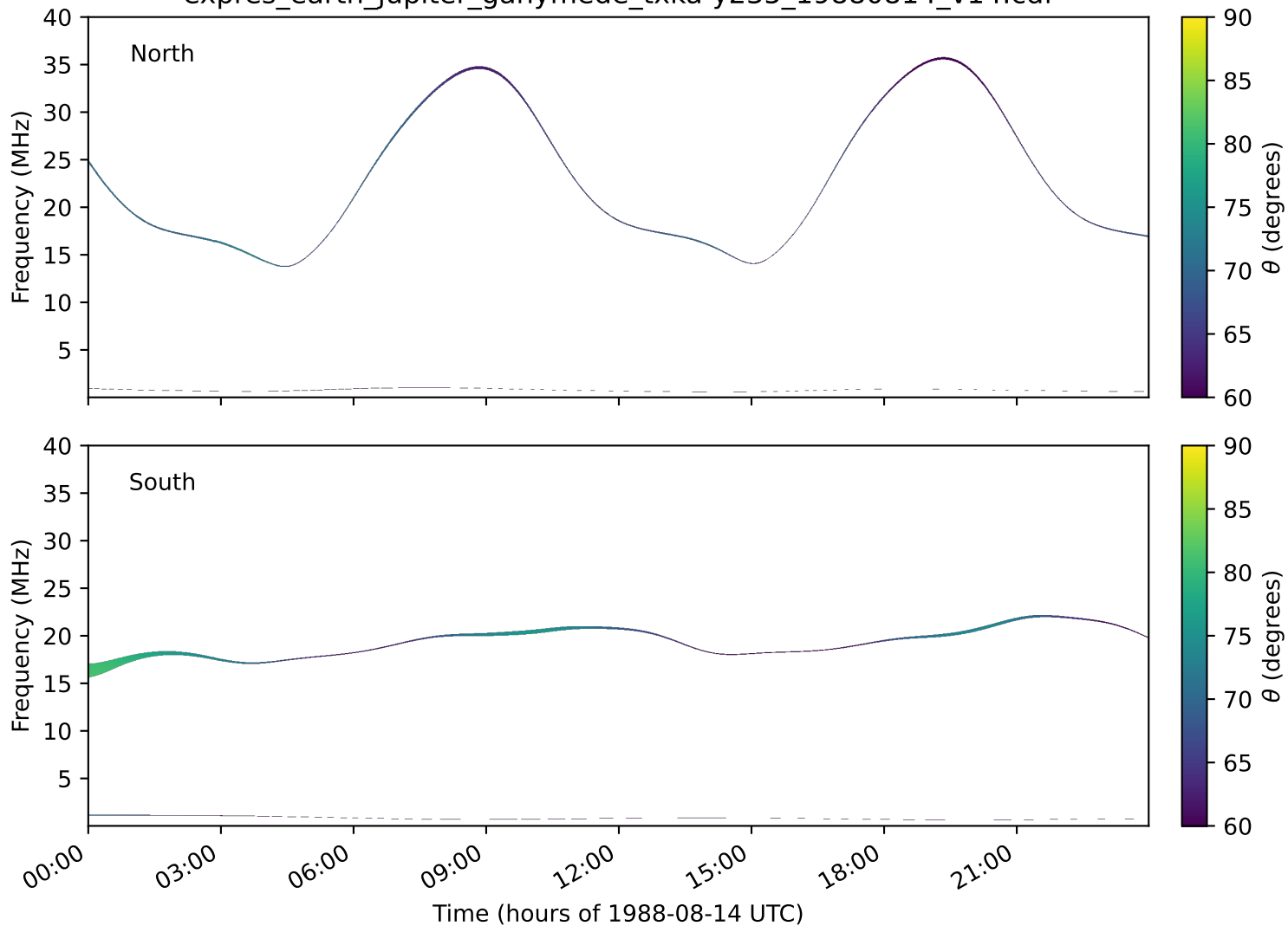
expres_earth_jupiter_ganymede_txka-y235_19880814_v14.cdf
