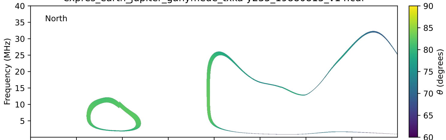
expres_earth_jupiter_ganymede_txka-y235_19880813_v14.cdf
