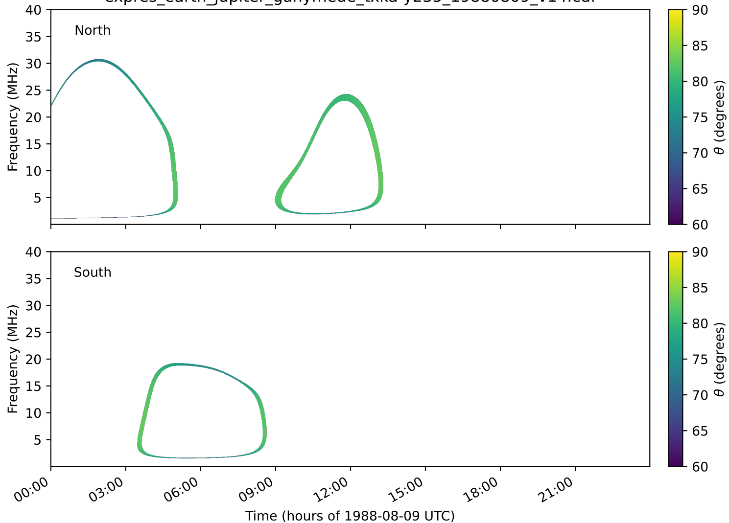
expres_earth_jupiter_ganymede_txka-y235_19880809_v14.cdf
