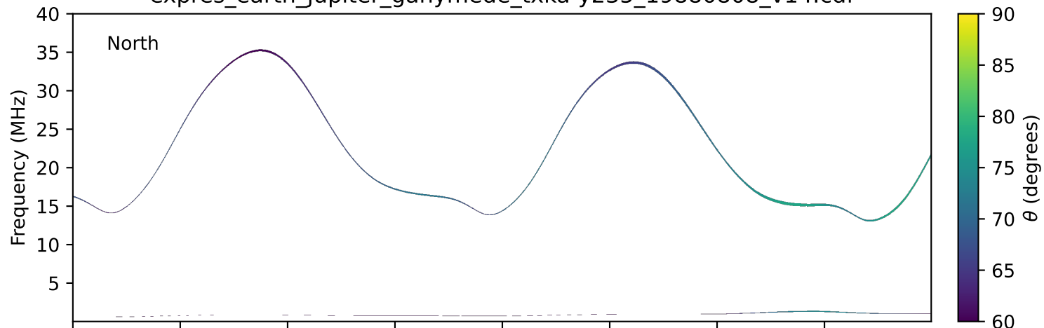
expres_earth_jupiter_ganymede_txka-y235_19880808_v14.cdf
