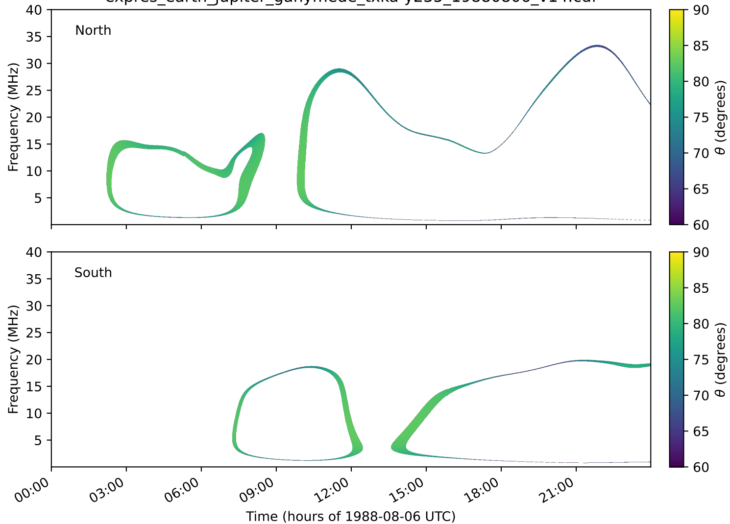
expres_earth_jupiter_ganymede_txka-y235_19880806_v14.cdf
