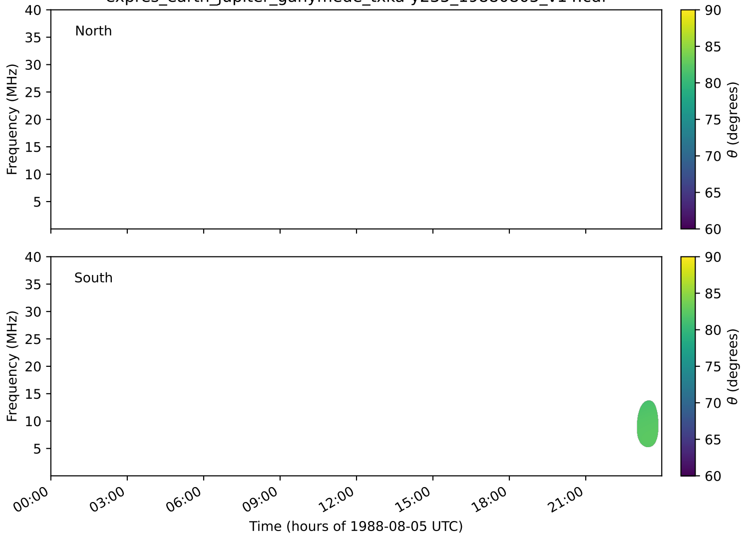
expres_earth_jupiter_ganymede_txka-y235_19880805_v14.cdf
